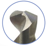
Fully ground 135° point angle Split point
