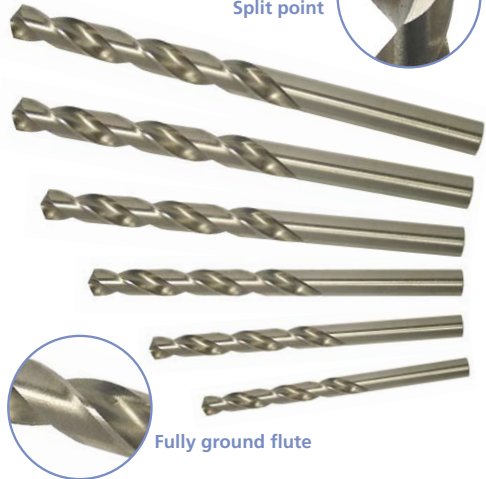
Fully ground 135° point angle Split point
